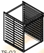
GN 2/1 Tepsi Kiti / GN 2/1 Tray Kit
